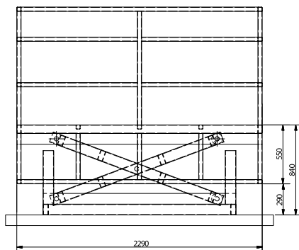
DVIG PLOŠČADI LIFTING THE PLATFORM
