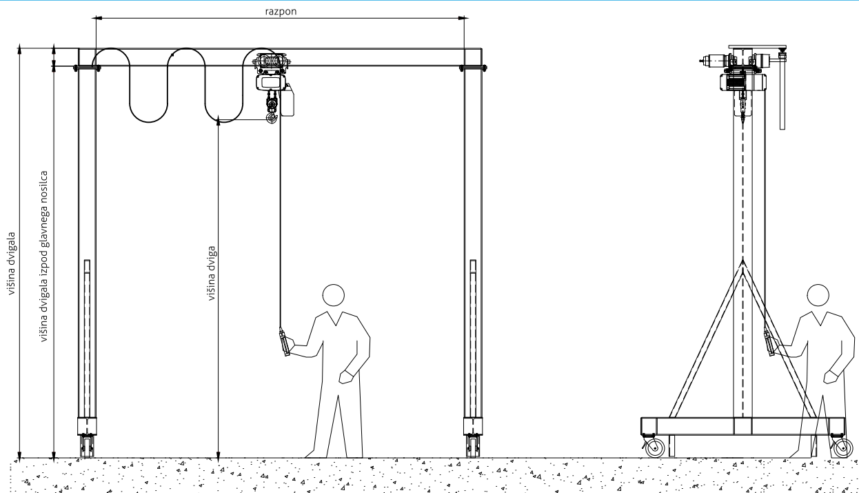
Višina dviga in nosilnost glede na potrebe / Lifting height and capacity according to the needs
